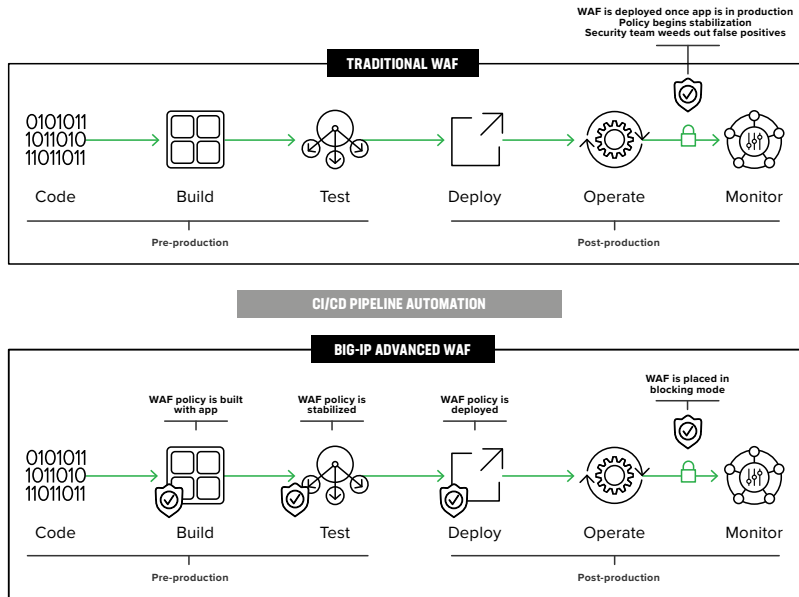
Figure 1: Incorporating WAF policy construction earlier in the development process reduces the risk of security misconfiguration late in the CI/CD pipeline.
